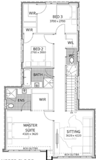
UPPER FLOOR
