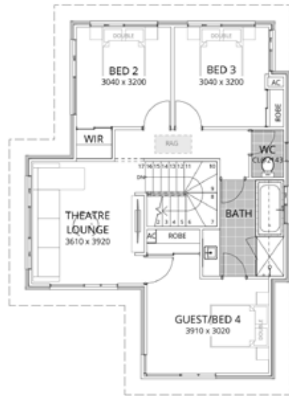
UPPER FLOOR
